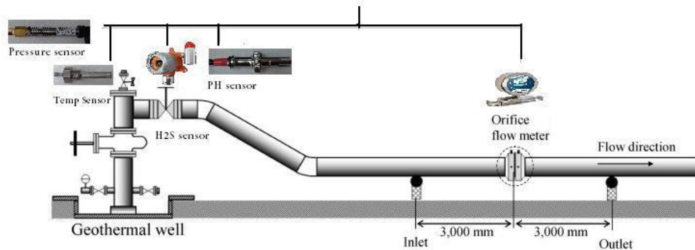
Application Diagram
